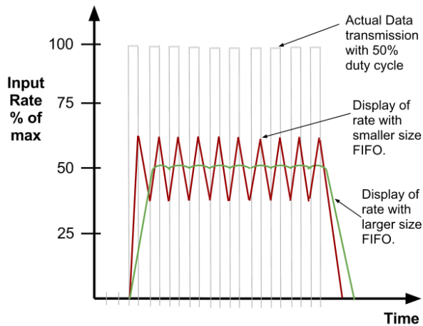
Figure 8. Graph showing effects of FIFO sizing
