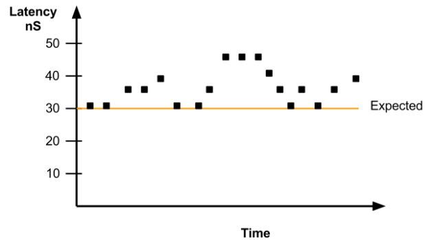
Figure 4. Graph showing observed latency issue
