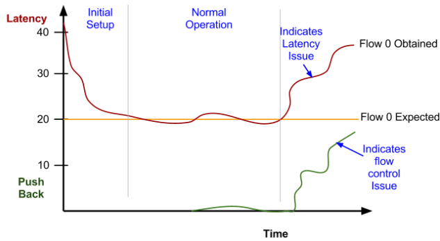
Figure 5. Graph showing latency along with flow control
