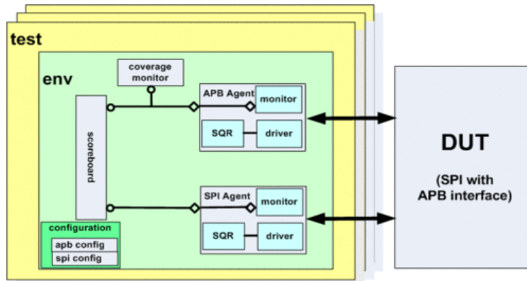
Figure 1 – A basic UVM Environment
