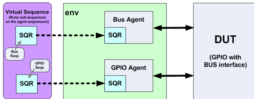
Figure 4 – The Virtual Sequence
