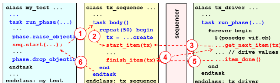
Figure 3 – Test/sequence/driver handshaking
