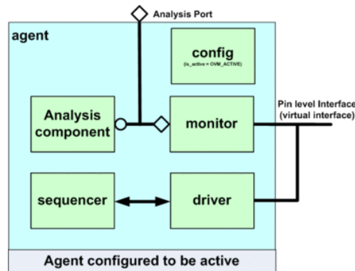
Figure 2 – A typical UVM Agent
