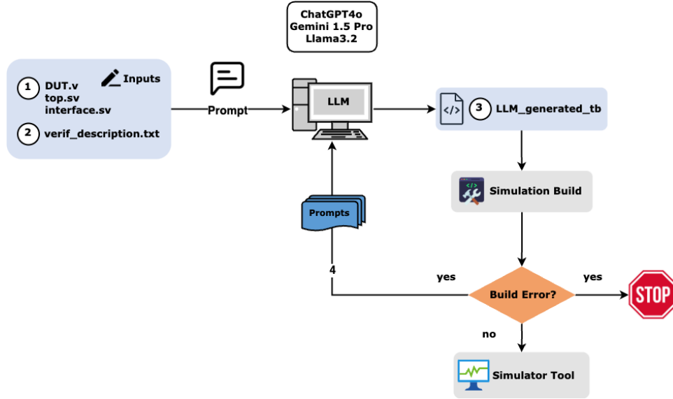
Fig. 1: LLM TB Generation to Build Flow
