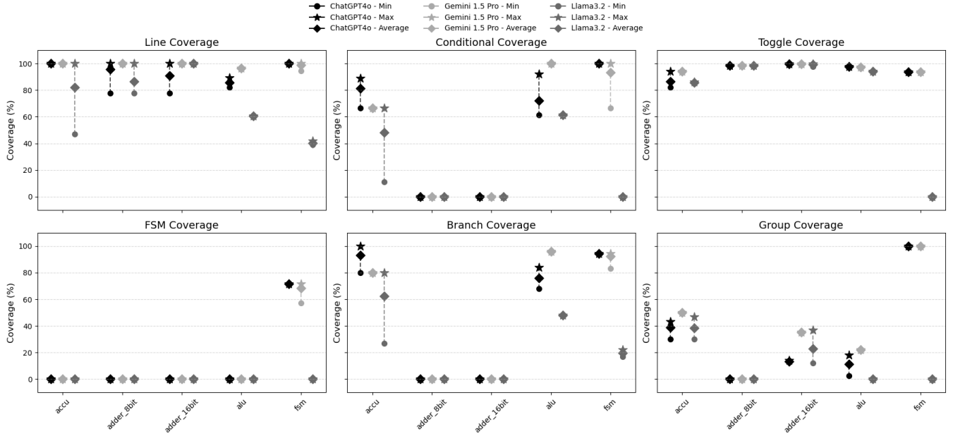
Fig. 7: Coverage Metrics across all LLMs and DUTs
